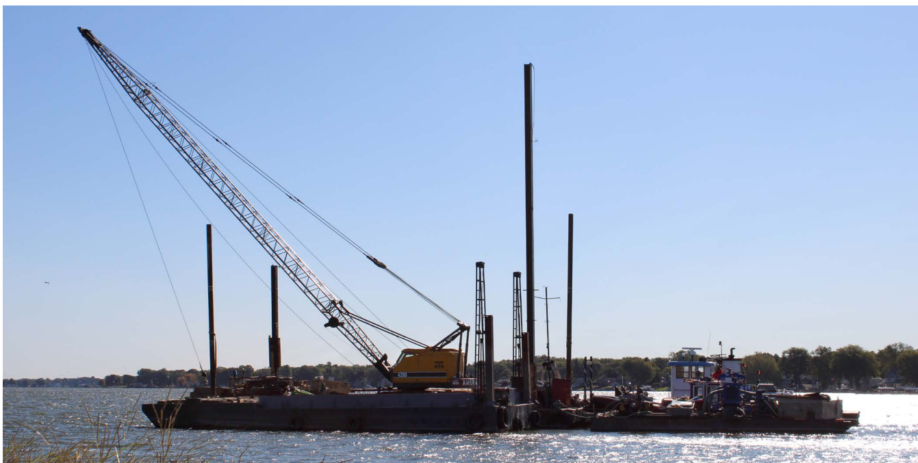
Figure 8 | Typical crane and/or deck barge
